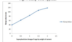
Fig. 2: Graph Between W/C Ratio 0.45 and Slump of Concrete With Adding Superplasticizer
